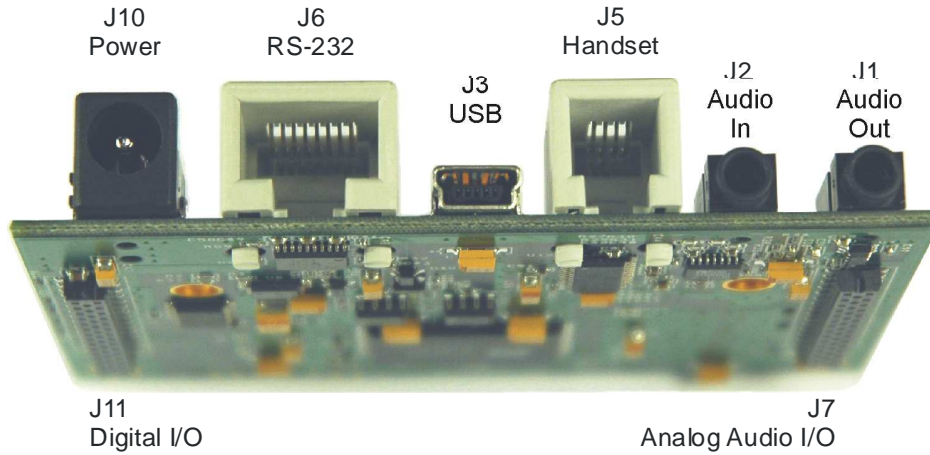
Figure 2 VC-55™- PR Vocoder Board Top
