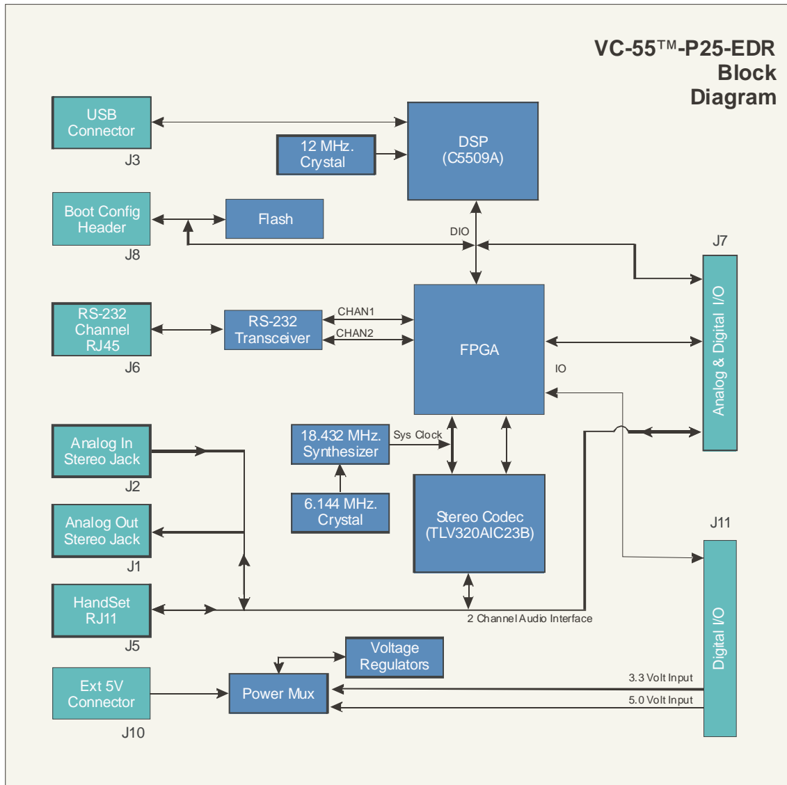
Figure 1 Block Diagram
